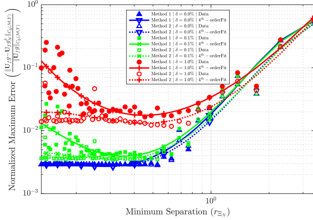
Fig. 9 Log-log plot of the normalized maximum prediction error versus the minimum separation distance r_{\Xi_N} , comparing Method 1 and Method 2 under three levels of deterministic sinusoidal uncertainty: 0%, 0.1%, and 1%. The number of quadrature points is fixed at M_q = 60 . Each marker represents the normalized maximum error computed at a given r_{\Xi_N} . Filled markers represent Method 1, while unfilled markers represent Method 2. Solid and dotted curves with markers correspond to fourth-order polynomial fits in the log-log scale for each method and uncertainty level.
