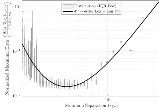
Fig. 4 Log-log plot of the normalized maximum prediction error versus the minimum separation distance r_{\Xi_N} , computed using Method 1 under zero-mean stochastic measurement uncertainty with a magnitude of 0.2%. For each r_{\Xi_N} , the corresponding boxplot shows the distribution of normalized maximum errors over 200 simulations. The solid curve represents a fourth-order polynomial fit of the average error in the log-log scale. Results are shown for the Gaussian kernel
