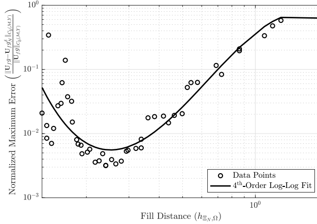
Fig. 5 Log-log plot of the normalized maximum prediction error versus the fill distance h_{\Xi_N, \Omega} , computed along 100 manifolds generated from initial conditions uniformly spaced along the x_2 axis from (1, 1) to approximately (1, 1.99) , approaching the singular point at (1, 2) . The simulation was performed using Method 1 under deterministic sinusoidal measurement uncertainty with a magnitude of 0.01%. Each marker corresponds to the normalized maximum error, and the solid curve represents a fourth-order polynomial fit in the log-log scale. Results are shown for the Gaussian kernel (103)
