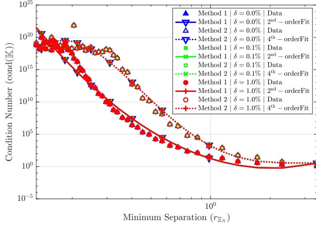
Fig. 10 Log-log plot of the condition number of the Grammian matrix versus the minimum separation distance r_{\Xi_N} , comparing Method 1 and Method 2 under three levels of deterministic sinusoidal measurement uncertainty: 0%, 0.1%, and 1%. The number of quadrature points is fixed at M_q = 60 . Each marker represents the condition number evaluated at a given r_{\Xi_N} . Filled markers represent the results of Method 1, and unfilled markers represent the results of Method 2. Solid and dotted curves with markers correspond to second-order and fourth-order polynomial fits in the log-log scale for Method 1 and Method 2, respectively
