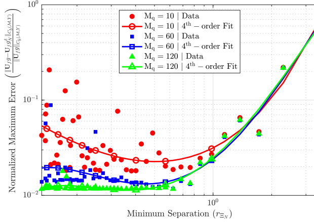
Fig. 8 Log-log plot of the normalized maximum prediction error versus the minimum separation distance r_{\Xi_N} , computed using Method 2 for three different numbers of quadrature points M_q = 10, 60, 120 , under deterministic sinusoidal measurement uncertainty of magnitude 0.1%. Each filled marker represents the normalized maximum error computed at a given r_{\Xi_N} . Solid curves with unfilled markers represent fourth-order polynomial fits in the log-log scale for each corresponding quadrature point setting
