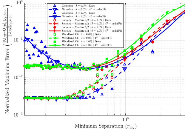
Fig. 6 Log-log plot of the normalized maximum prediction error versus the minimum separation distance r_{\Xi_N} , computed using Method 1 with three different kernel functions: Gaussian, Sobolev–Matérn 5/2, and Wendland C6; see [34, pp. 54–57]. Each marker represents the normalized maximum error computed under deterministic sinusoidal measurement uncertainty. Filled and unfilled markers represent measurement uncertainties with magnitudes of 1% and 0% (noise-free), respectively. Solid and dashed lines with unfilled markers represent fourth-order polynomial fits in the log-log scale for the 1% and noise-free cases, respectively.
