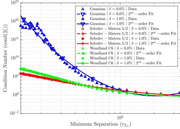
Fig. 7 Log-log plot of the condition number of the Grammian matrix \mathbb{K}_N versus the minimum separation distance r_{\Xi_N} , corresponding to Method 1 with three different kernel functions: Gaussian, Sobolev–Matérn 5/2, and Wendland C6; see [34, pp. 54–57]. Each marker represents the condition number evaluated under deterministic sinusoidal measurement uncertainty. Filled and unfilled markers represent measurement uncertainties with magnitudes of 1% and 0% (noise-free), respectively. Solid and dashed lines with unfilled markers represent second-order polynomial fits in the log-log scale for the 1% and noise-free cases, respectively
