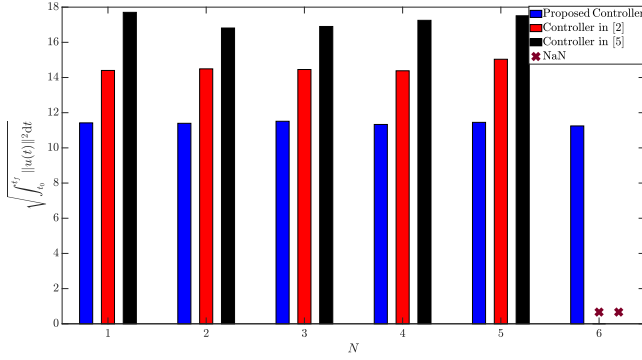
Fig. 4. l_2 -norm of the control effort for the same simulations employed to generate Figure 2. The proposed controller requires a significantly smaller control effort.
